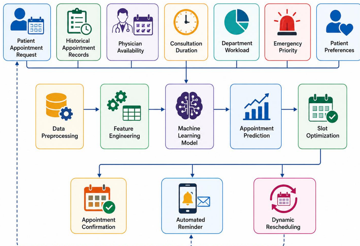
Figure 4- AI-Based Intelligent Appointment Scheduling Framework
